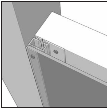
Clear Channel extrusion for side panel mounting
